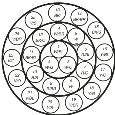
25 PAIR UNIT (U-25)
