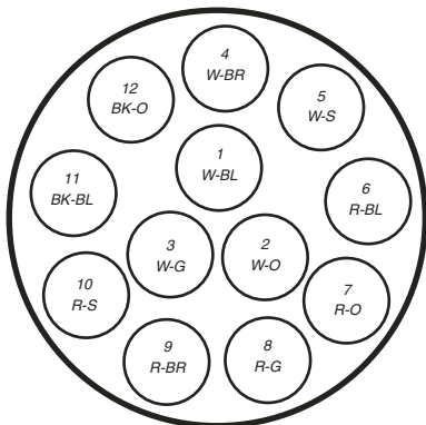
300 PAIR SUPER-UNIT FOR 4200 PAIR CABLE
